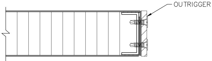
ANGLE OUTRIGGER MOUNTING BRACKET
