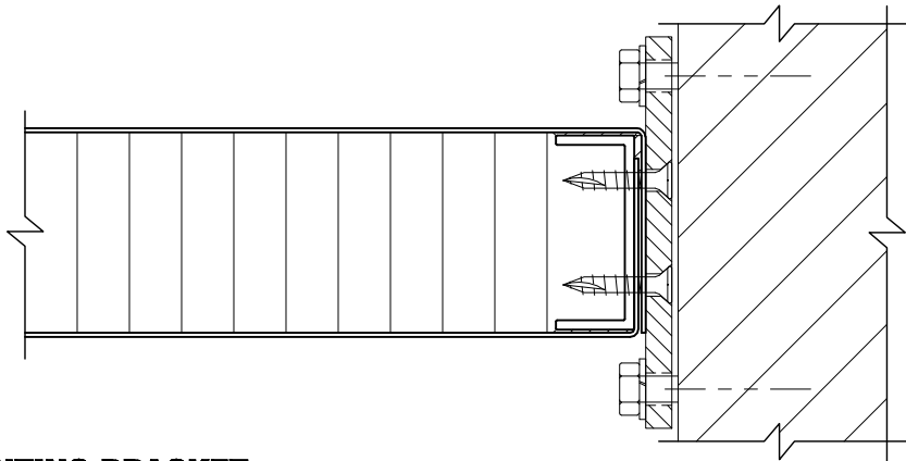
ANGLE WALL MOUNTING BRACKET
