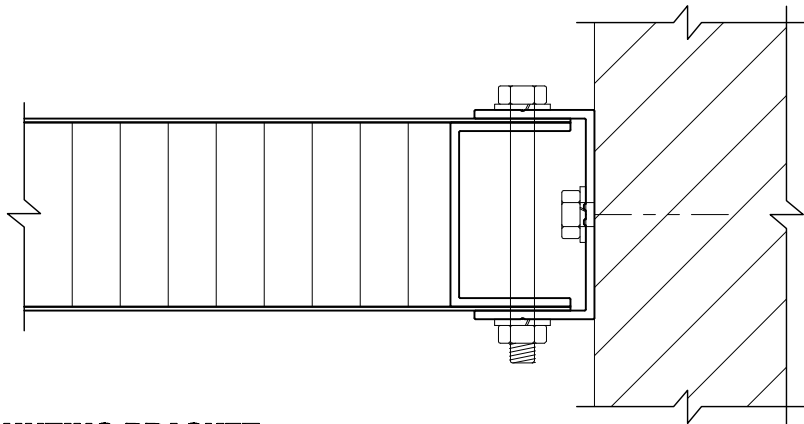
STANDARD WALL MOUNTING BRACKET
