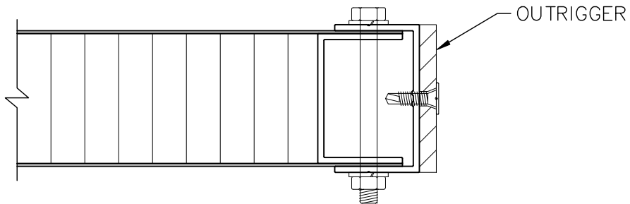
STANDARD OUTRIGGER MOUNTING BRACKET
