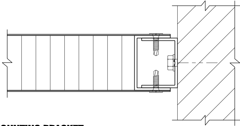
CONCEALED WALL MOUNTING BRACKET
